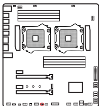
2-1 Clear CMOS Jumper CLR-CMOS
