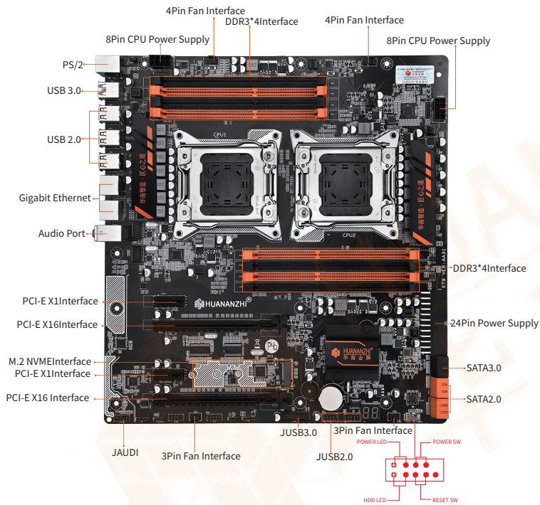
1-1 X79 Dual-8D Motherboard illustration
